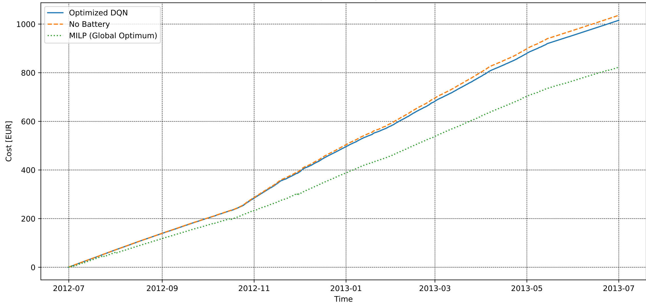
User 81 - Basic Training - Electricity Cost [DQN vs MILP]
